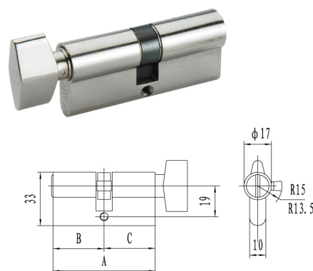
■ 标准B型卫生间锁芯 WASHROOM KNOB CYLINDER MODEL B
