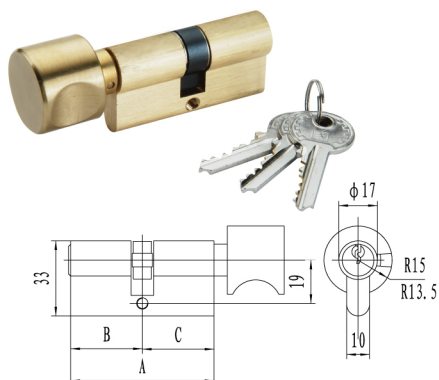
■ 标准D型手轮锁芯 PROFILE KNOB CYLINDER MODEL D
