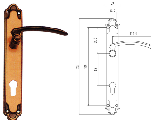
ZAMAK HANDLE REF.450Y FINISH: AB,AC
