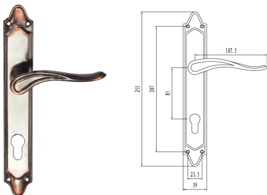
ZAMAK HANDLE REF.300Y FINISH: AB,AC
