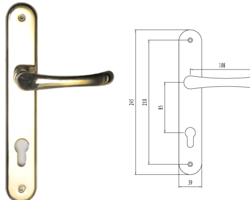
ZAMAK HANDLE REF.BH001 FINISH: GOLDEN, CHROME
