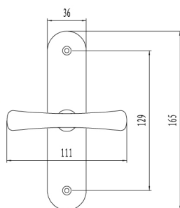
ZAMAK HANDLE REF.215-WH
