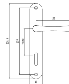
ZAMAK HANDLE REF.215K
