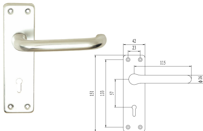
ALU.HANDLE REF.141K FINISH: GOLDEN, SILVER, BRONZE
