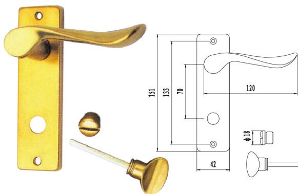
ALU.HANDLE REF.125WC FINISH: GOLDEN, SILVER, BRONZE
