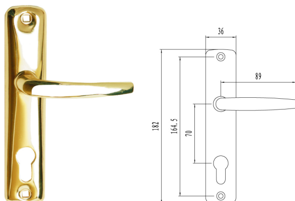
ZAMAK HANDLE REF.124 FINISH: CHROME, GOLDEN
