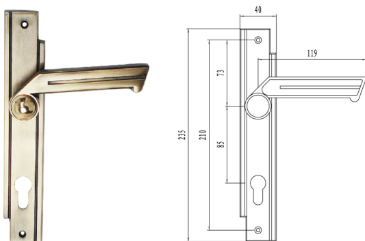
ZAMAK HANDLE REF.500PB FINISH: AB,AC
