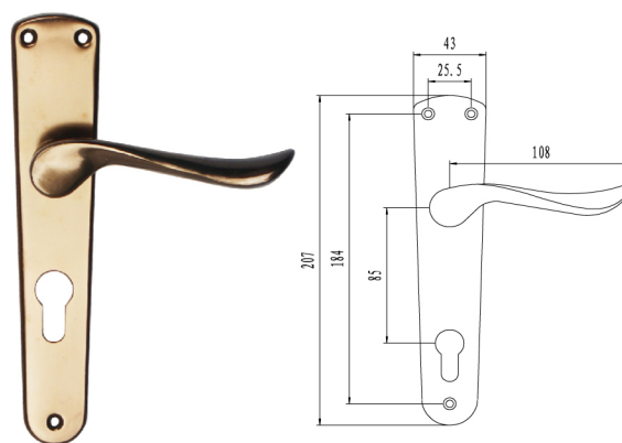
ALU.HANDLE REF.204 FINISH: SILVER, GOLDEN, BRONZE
