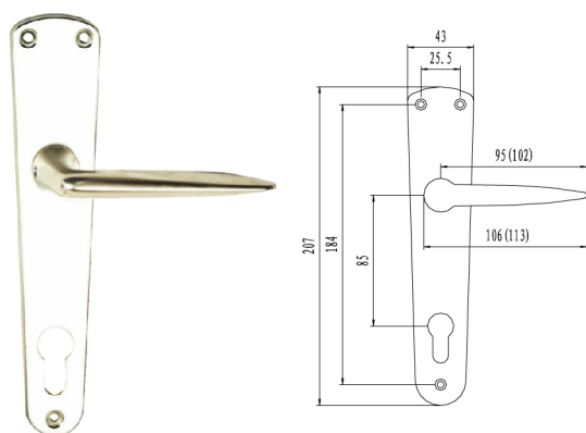
ALU.HANDLE REF.203W FINISH: SILVER, GOLDEN
