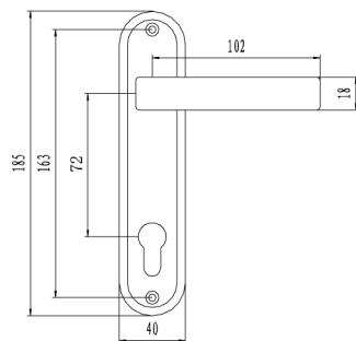
ALU.HANDLE REF.126
