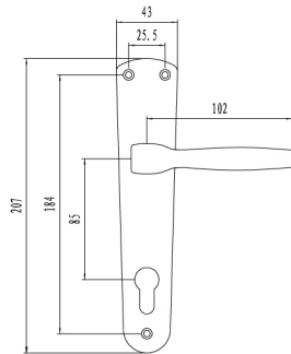
ALU.HANDLE REF.205
