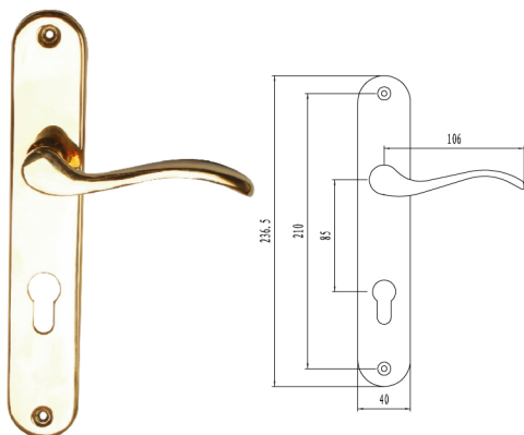
ZAMAK HANDLE REF.529 FINISH: GOLDEN, CHROME
