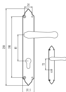
ZAMAK HANDLE REF.6001AB
