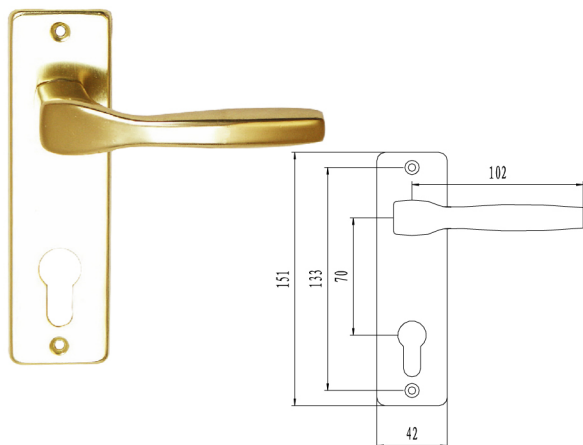
ALU.HANDLE REF.138 FINISH: GOLDEN, SILVER, BRONZE
