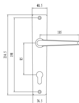
ALU.HANDLE REF.209
