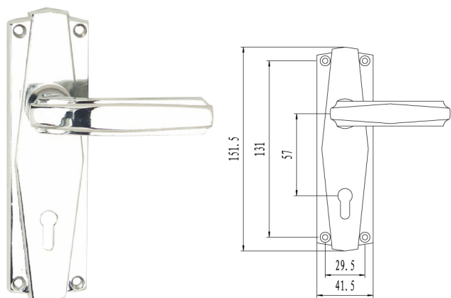
ZAMAK HANDLE REF.0223 FINISH: CHROME GOLDEN
