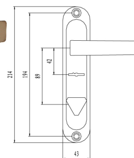
ZAMAK HANDLE REF.02-S
