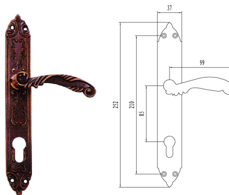
ZAMAK HANDLE REF.9011AC FINISH: AB,AC,AG
