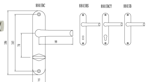
ALU.HANDLE REF.8803
