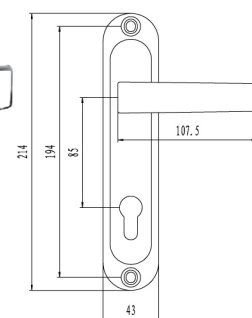
ZAMAK HANDLE REF.01-C
