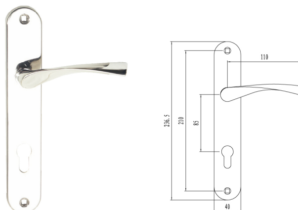
ZAMAK HANDLE REF.549 FINISH: CHROME GOLDEN
