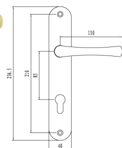
ZAMAK HANDLE REF.215
