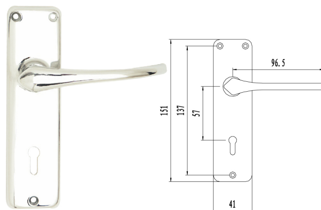
ZAMAK HANDLE REF.0226 FINISH: CHROME GOLDEN
