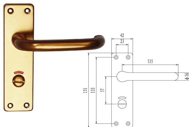
ALU.HANDLE REF.1141WC W/INDICATION FINISH: GOLDEN, SILVER, BRONZE
